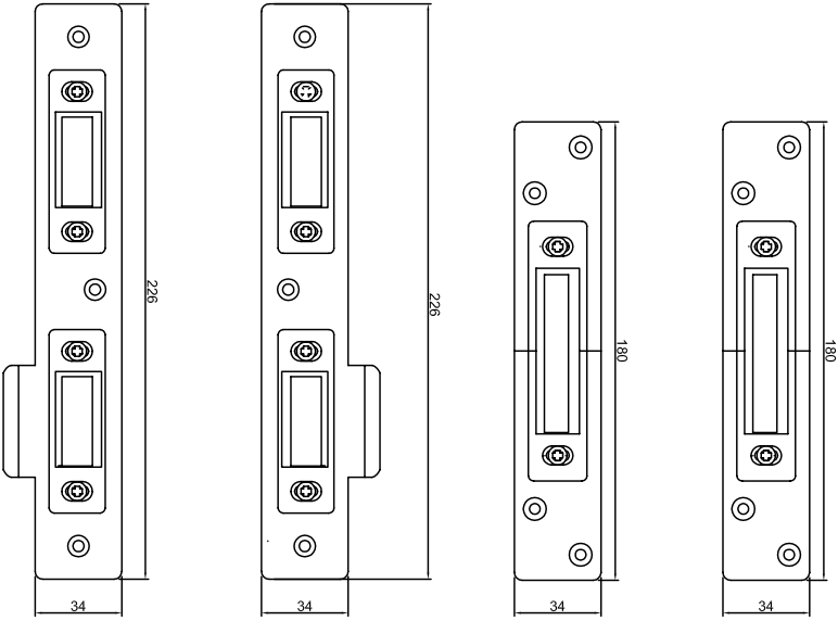
XLC0001-KE Centre Keep
