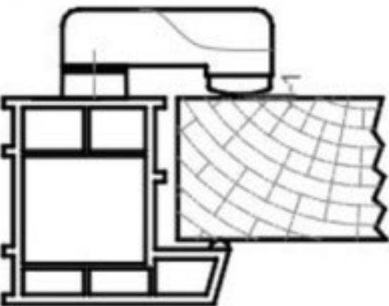
Typical Composite Flush Door Section
